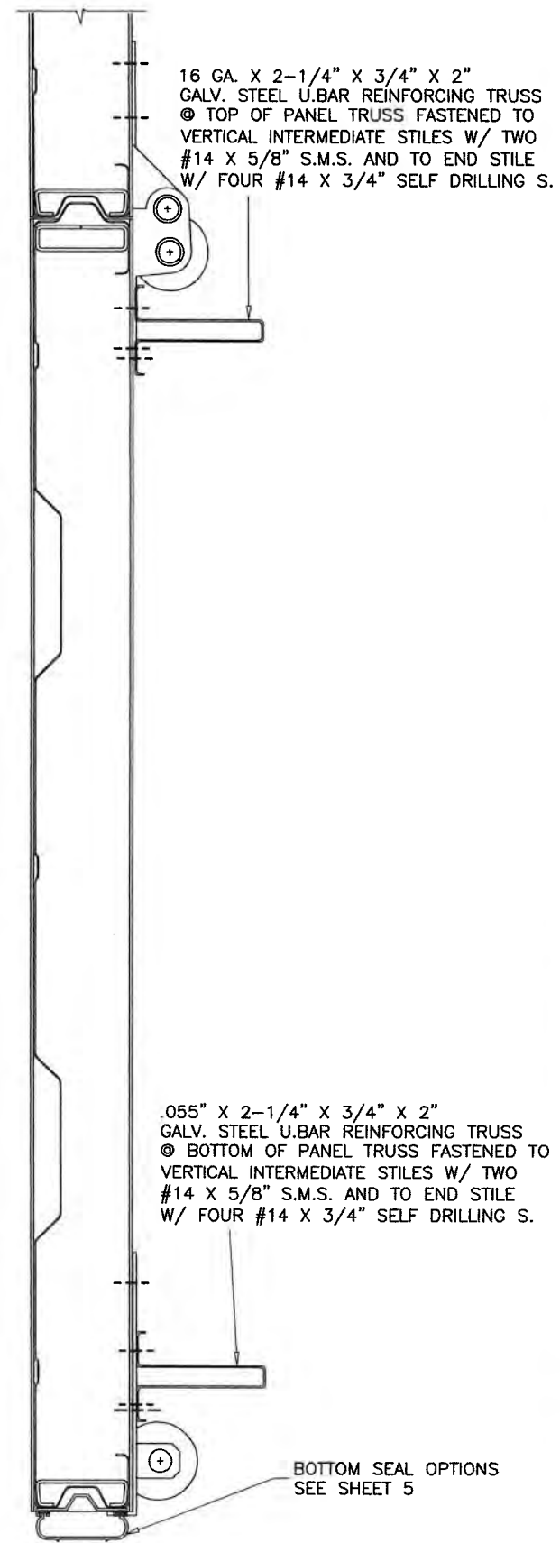
BOTTOM PANEL REINFORCING
